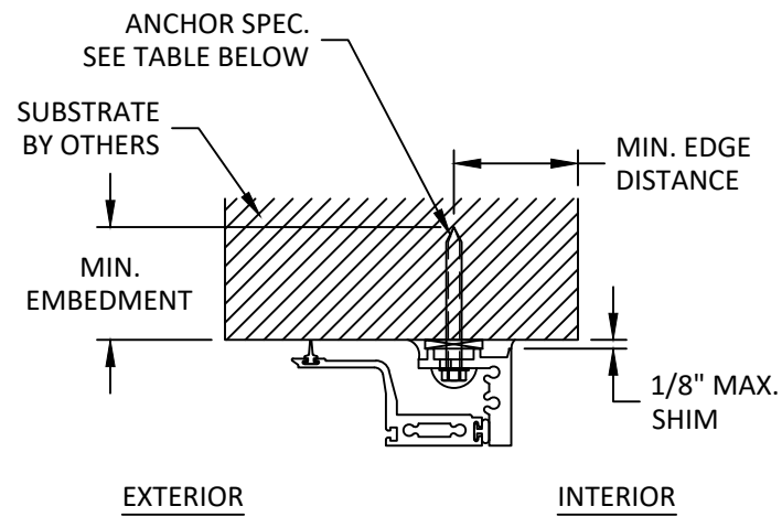
E 5 INSTALLATION DETAIL HEAD
