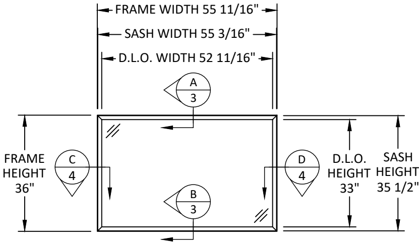
TYPICAL ELEVATION
