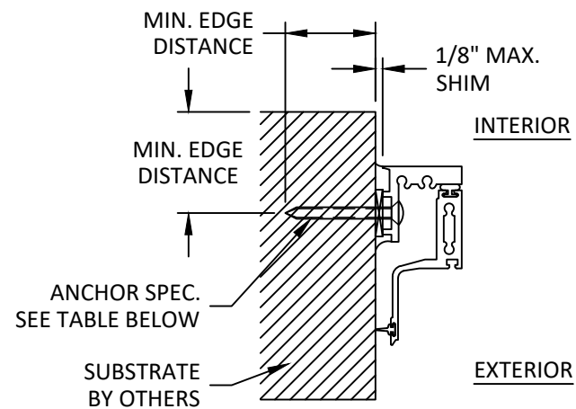
G 5 INSTALLATION DETAIL JAMB
