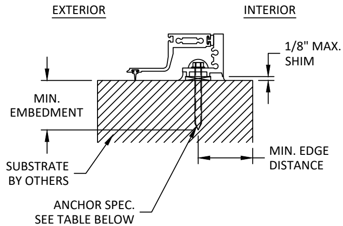
F 5 INSTALLATION DETAIL SILL
