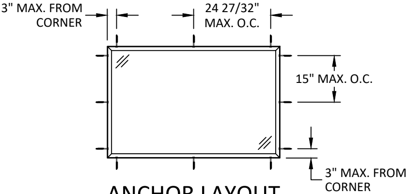
ANCHOR LAYOUT
